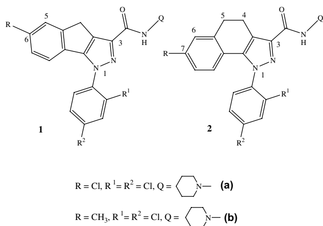
Figure 2. Homologous tricyclic pyrazolic CB-receptor ligands.
