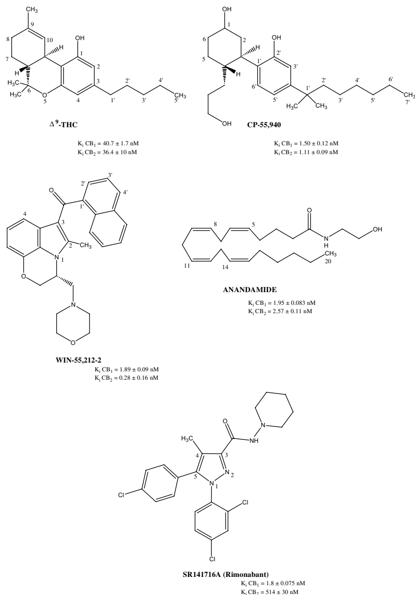
Figure 1. Cannabinoid receptor binder structures and their receptor affinities expressed as K_i .
