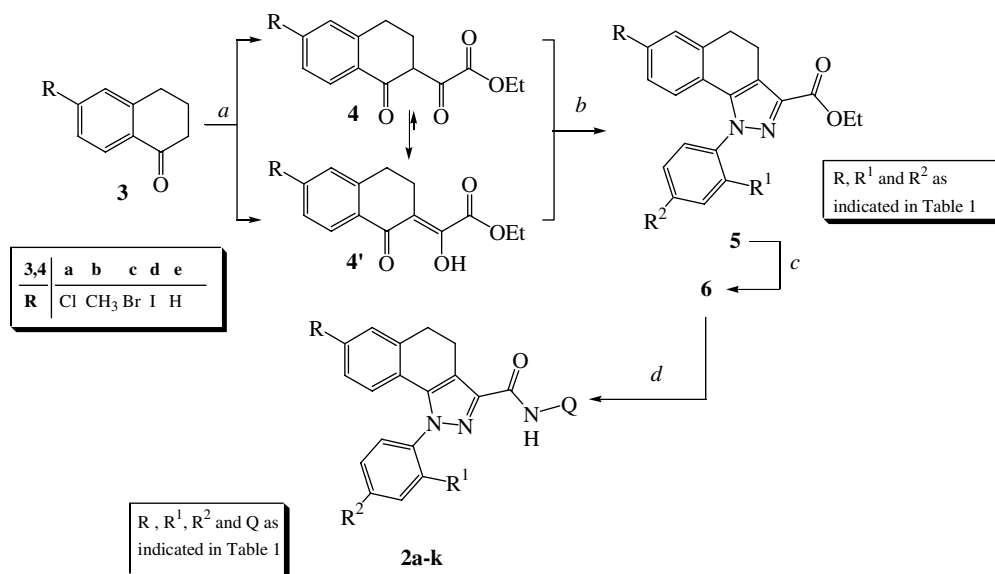
Scheme 1. Reagents and conditions: (a) Na, dry EtOH, (COOEt) 2 ; (b) ArNHNH 2 ·HCl, EtOH; (c) KOH, MeOH; (d) SOCl 2 , C 6 H 5 -CH 3 , CH 2 Cl 2 , TEA, Q-NH 2 .
